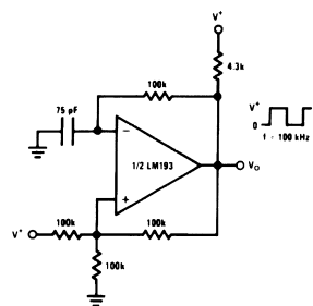
Figure 15. Driving CMOS
